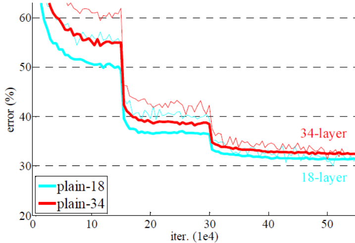
Error rates on ImageNet validation
