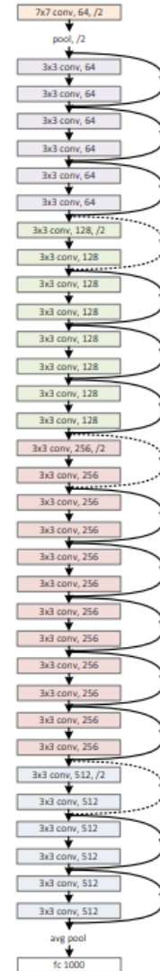
ResNet
